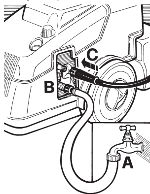
Raccordement hydraulique
